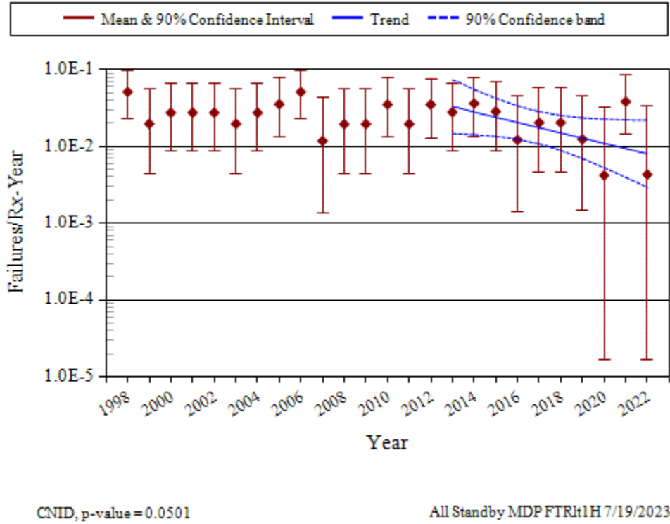
Figure 13. Frequency of FTR ≤1H events (events per reactor year) trend for standby MDPs.
