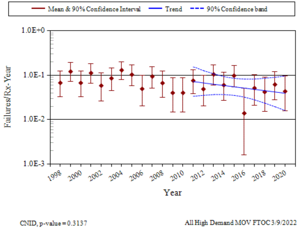
Figure 10. Frequency of FTQC events (failures per reactor year) for high-demand MOVs.
