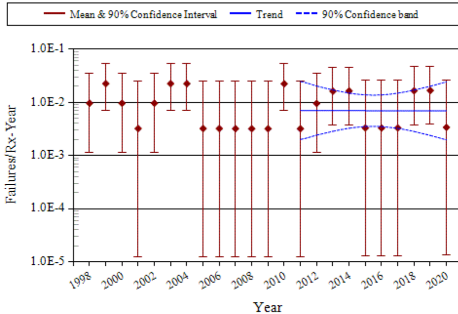
Figure 11. Frequency of FTOP events (failures per reactor year) for low-demand MOVs.
