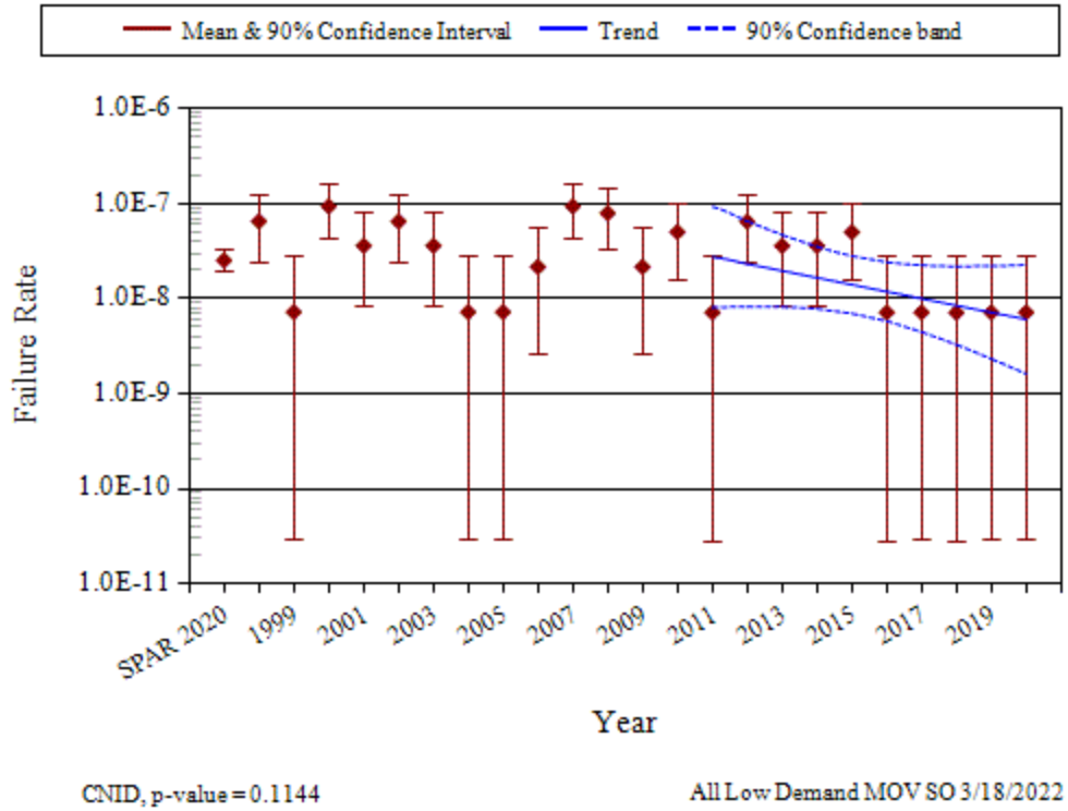
Figure 5. Failure rate estimate trend for low-demand MOV SO.
