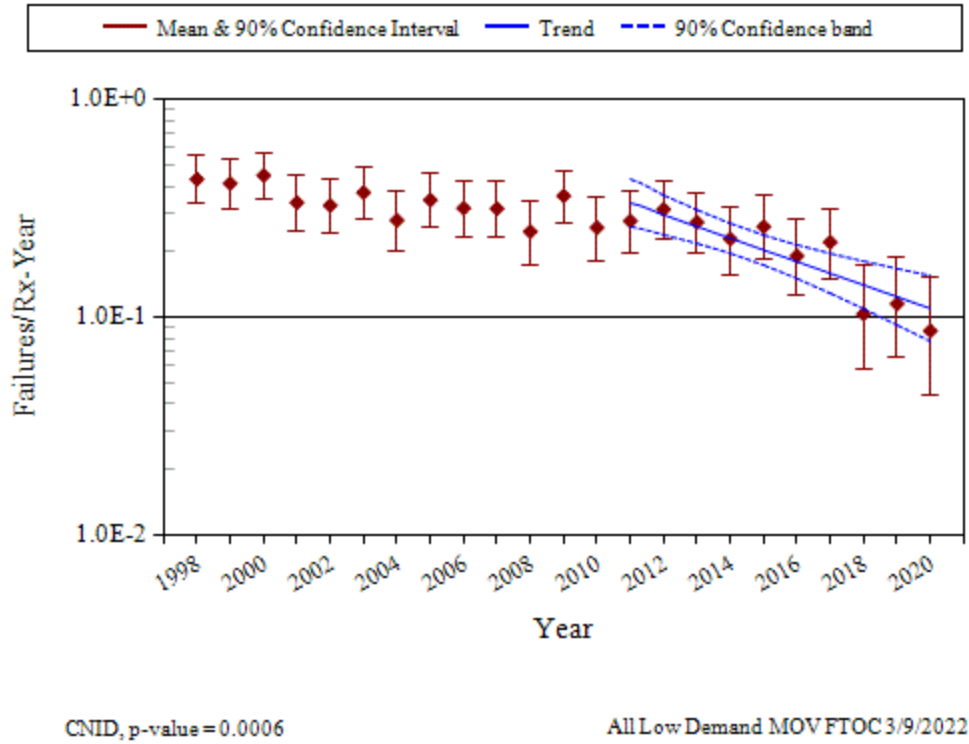
Figure 9. Frequency of FTQC events (failures per reactor year) for low-demand MOVs.
