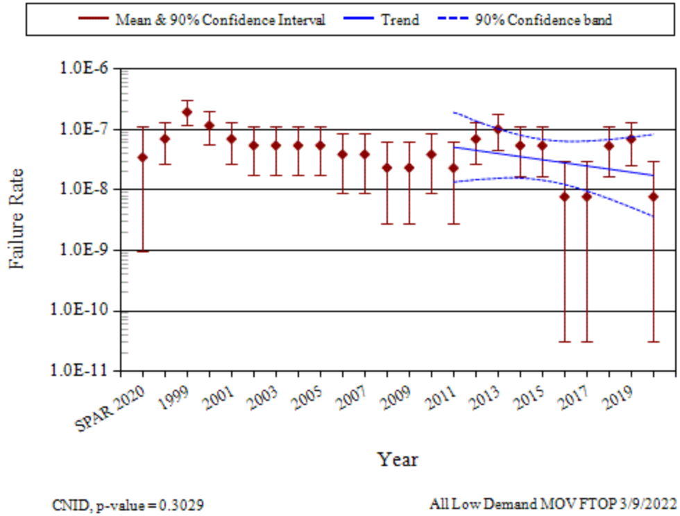
Figure 3. Failure rate estimate trend for low-demand MOV FTOP.
