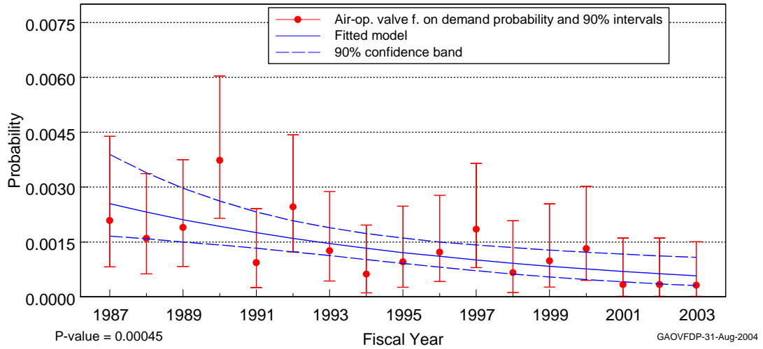
Figure 1. Air-operated valves failure on demand.
