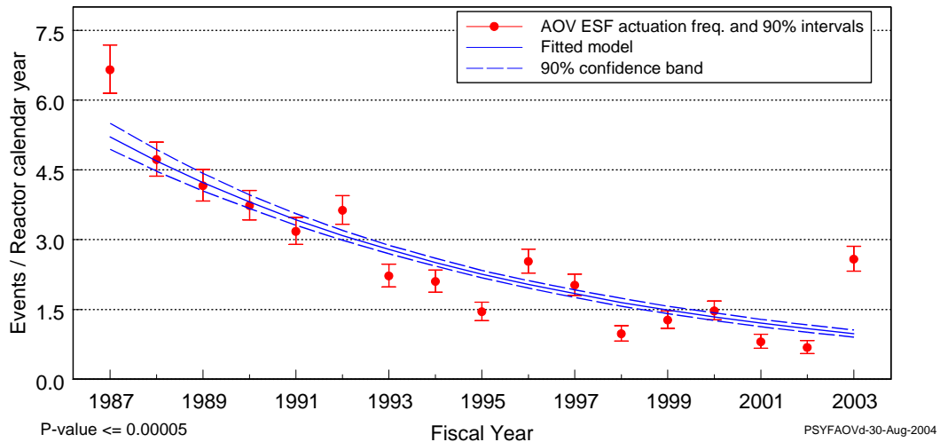
Figure 4. Frequency (events per operating year) of unplanned demands, as a function of fiscal year.
