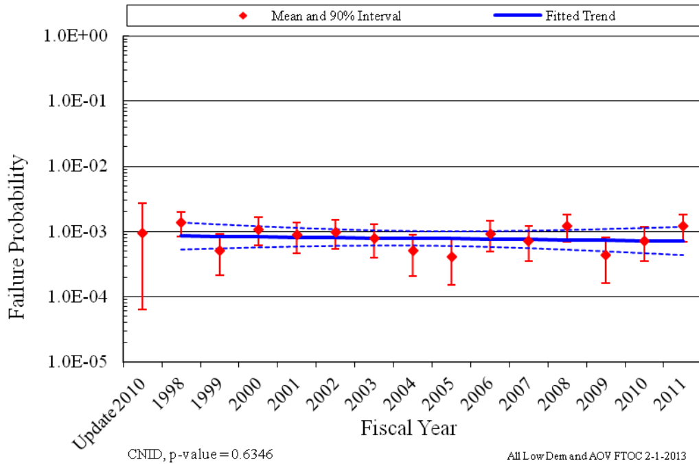
Figure 1. Failure probability estimate trend for AOV FTOC, all systems, industry-wide trend of AOVs with \leq 20 demands per year.
