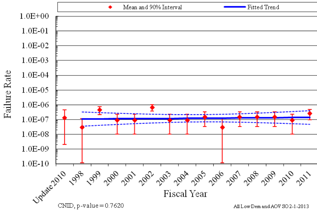
Figure 5. Failure rate estimate trend for AOV SO, all systems, industry-wide trend of AOVs with \leq 20 demands per year.
