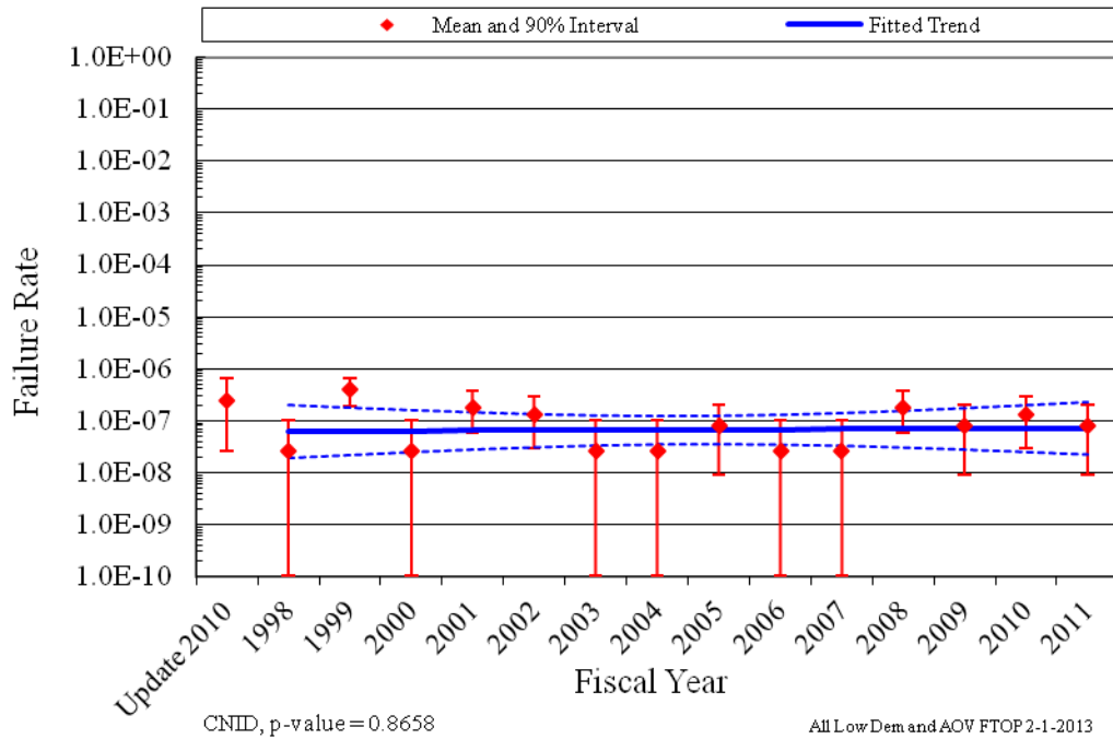
Figure 3. Failure rate estimate trend for AOV FTOP, all systems, industry-wide trend of AOVs with \leq 20 demands per year.
