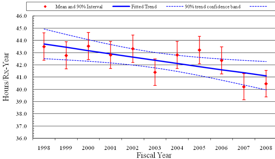
Figure 11. Frequency (events per reactor year) of start demands, EPS and HPCS EDGs.
