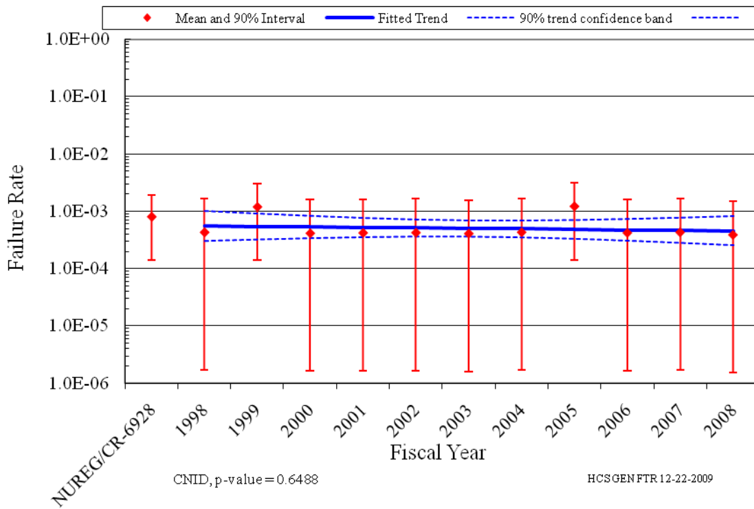
Figure 6. HPCS, industry-wide EDG FTR>1H trend.
