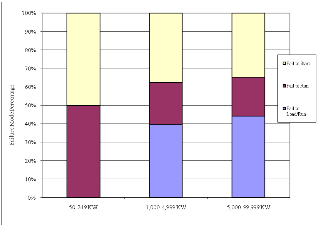
Figure 21. EPS EDG component failure modes by EPS EDG rating.
