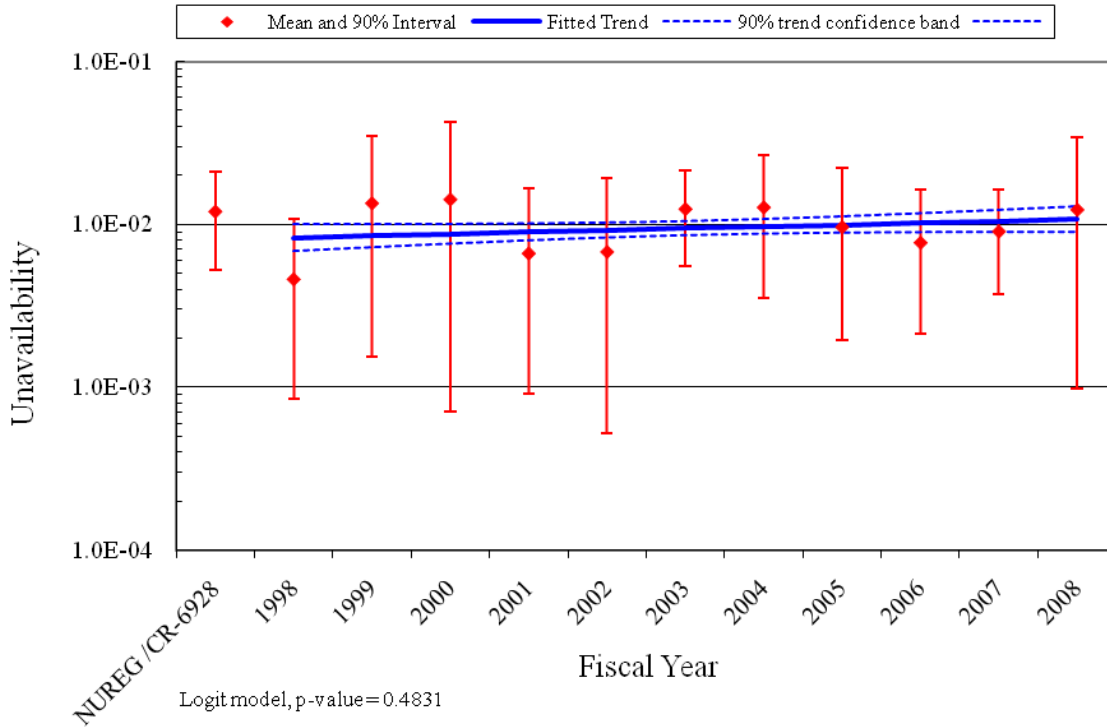
Figure 8. HPCS EDG UA trend.
