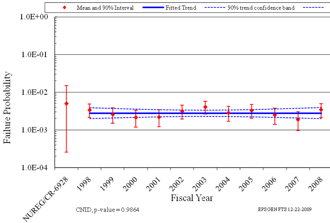
Figure 1. EPS, industry-wide EDG FTS trend.
