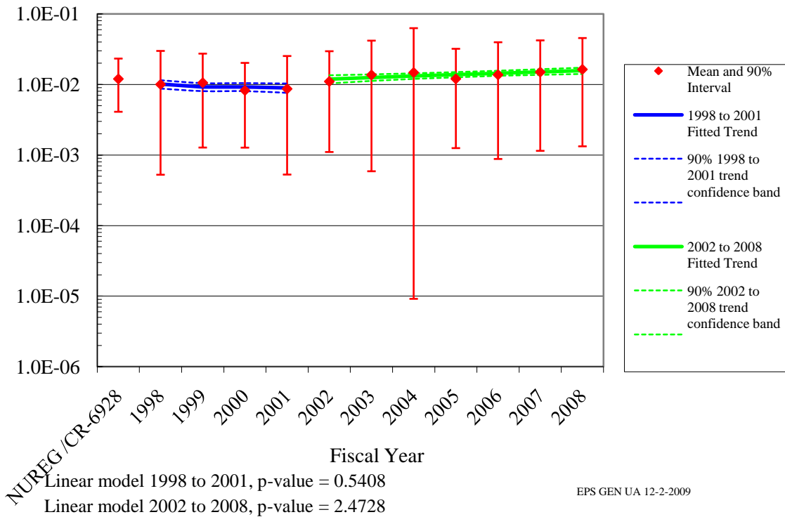
Figure 7. EPS EDG UA trend.
