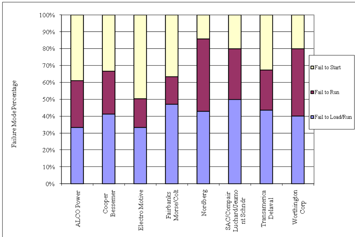
Figure 20. EPS EDG failure distribution by manufacturer.
