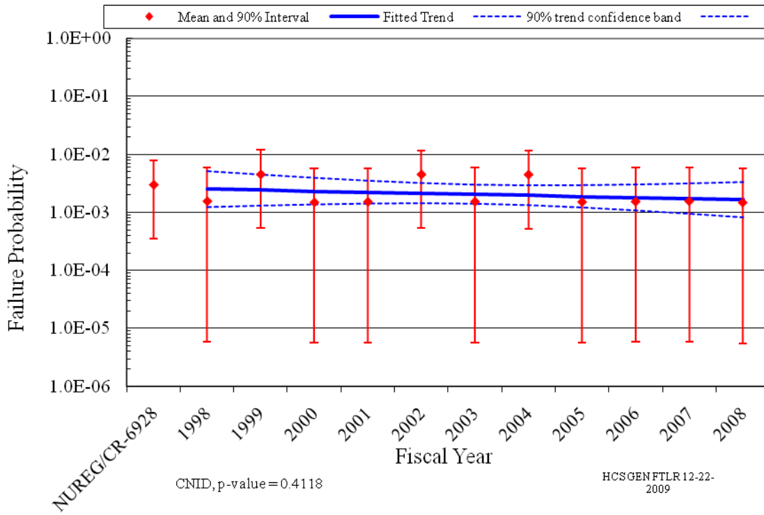
Figure 4. HPCS, industry-wide EDG FTS trend.
