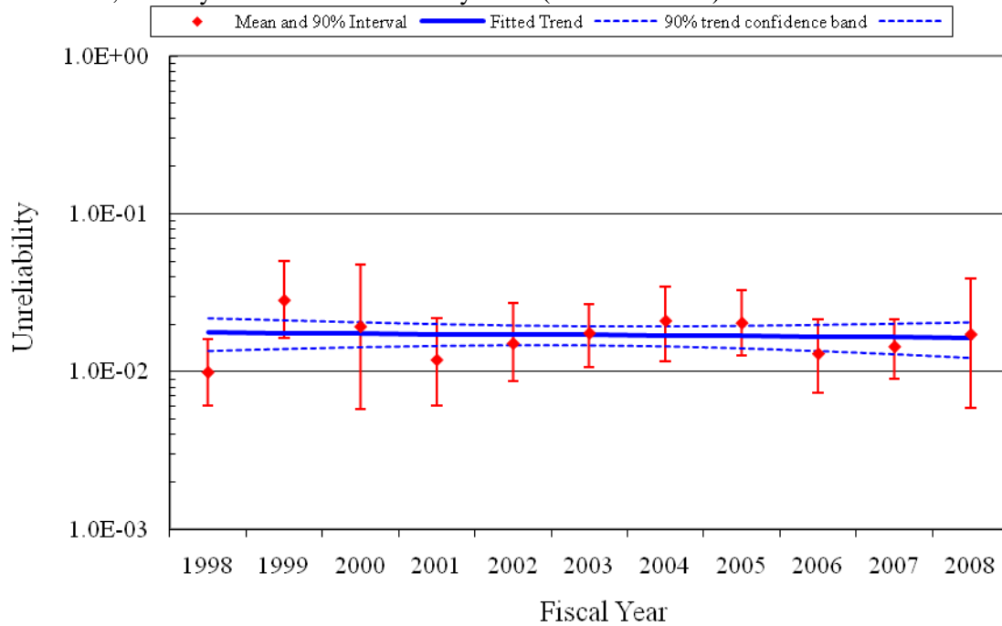
Figure 9. EPS, industry-wide EDG unreliability trend (8-hour mission).
