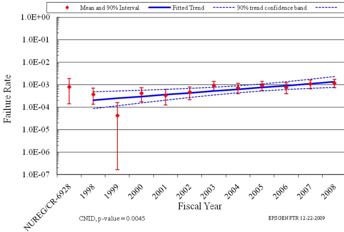
Figure 3. EPS, industry-wide EDG FTR>1H trend.
