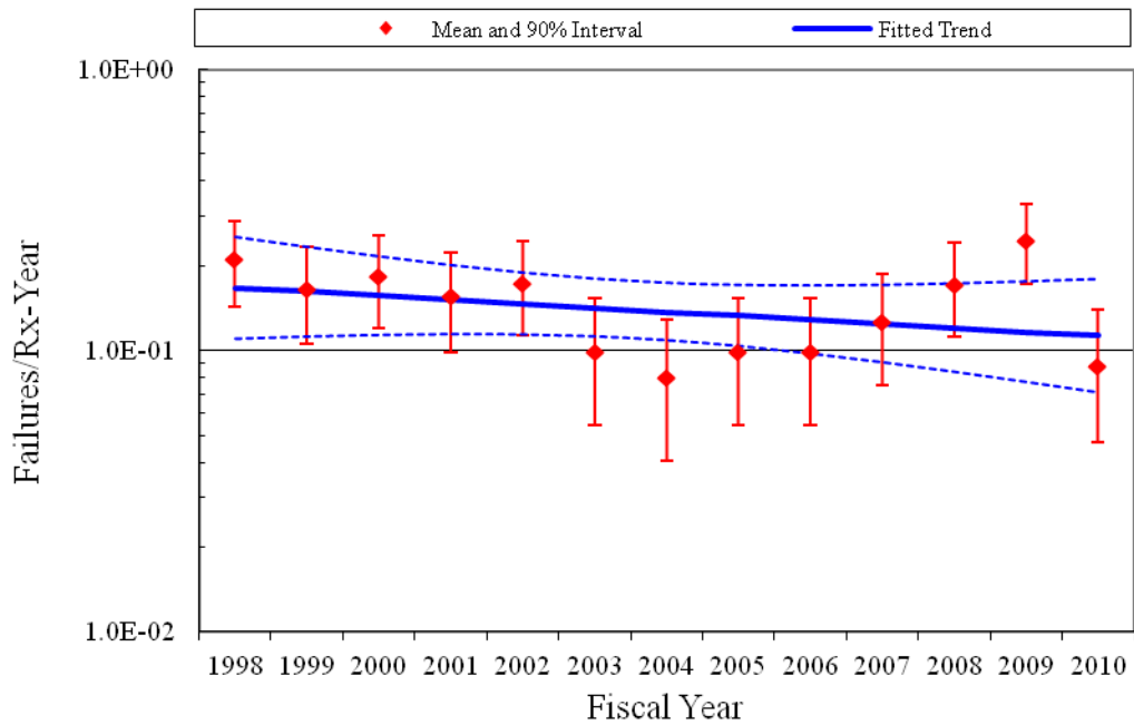
Figure 17. Frequency (failures per reactor year) of FTS events, normally running MDPs.
