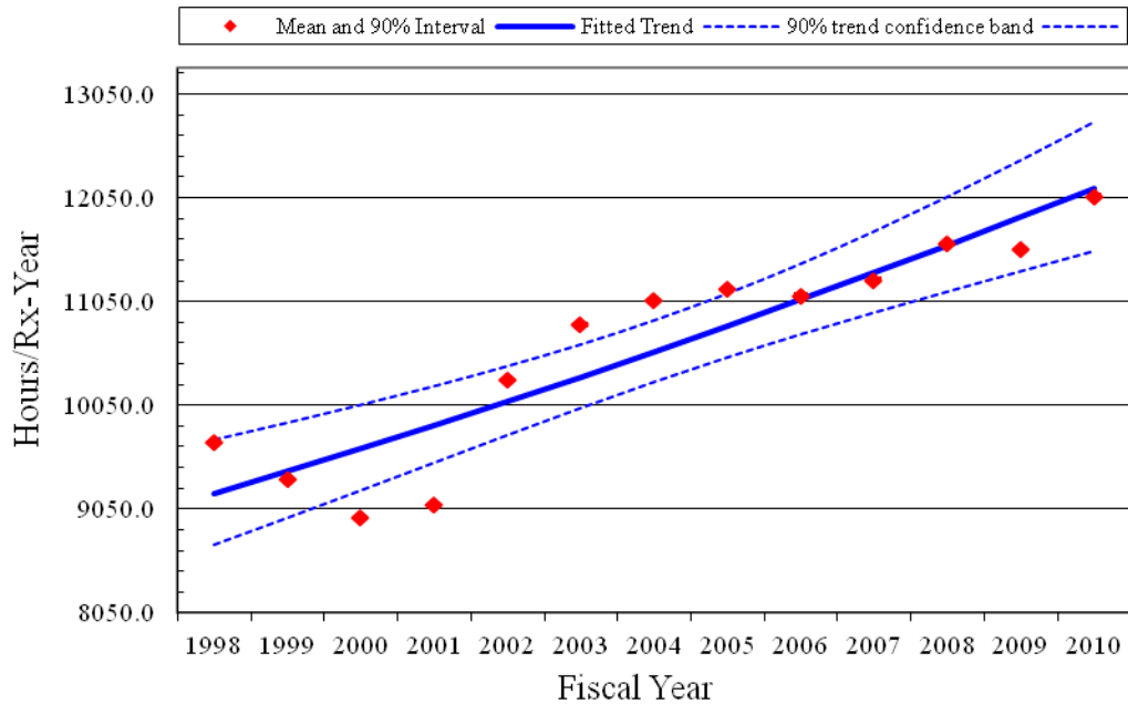
Figure 10. Standby MDP run hours per reactor critical year of run \leq 1H hours.
