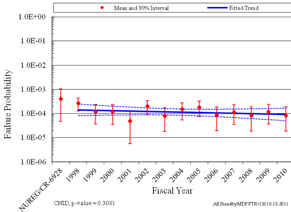
Figure 2. Standby systems, industry-wide MDP FTR ≤ 1H trend.
