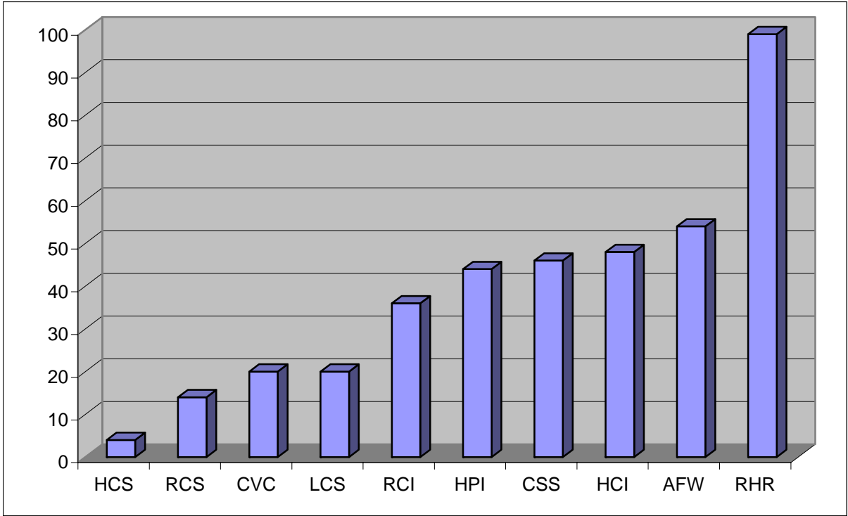
Figure 7. MOV system failures distribution
