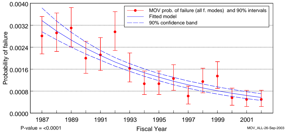
Figure 1. Motor-operated valves failure on demand.
