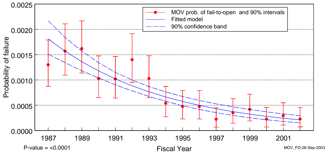
Figure 2. Motor-operated valves fail-to-open.
