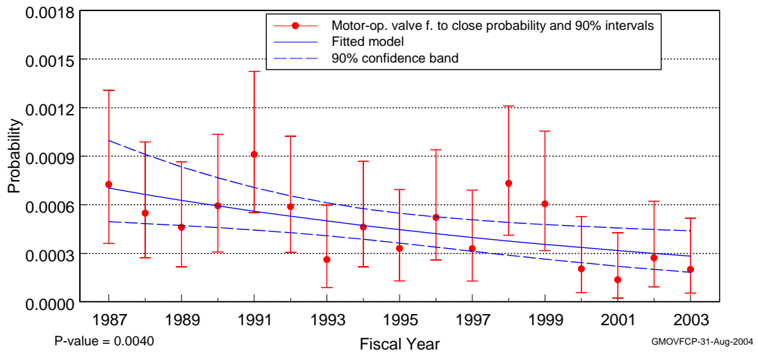
Figure 3. Motor-operated valves fail-to-close.
