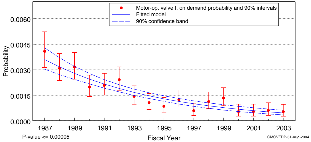
Figure 1. Motor-operated valves failure on demand.
