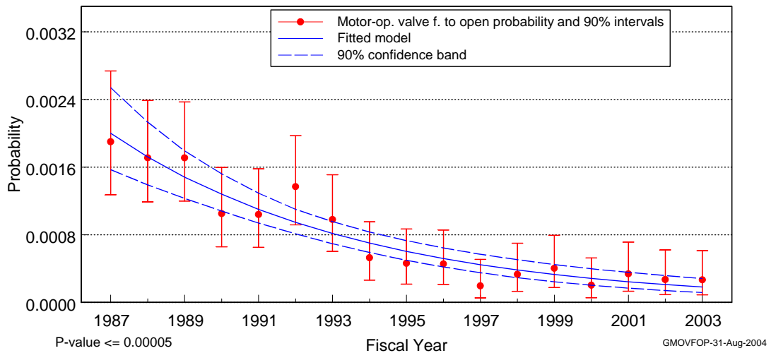
Figure 2. Motor-operated valves fail-to-open.
