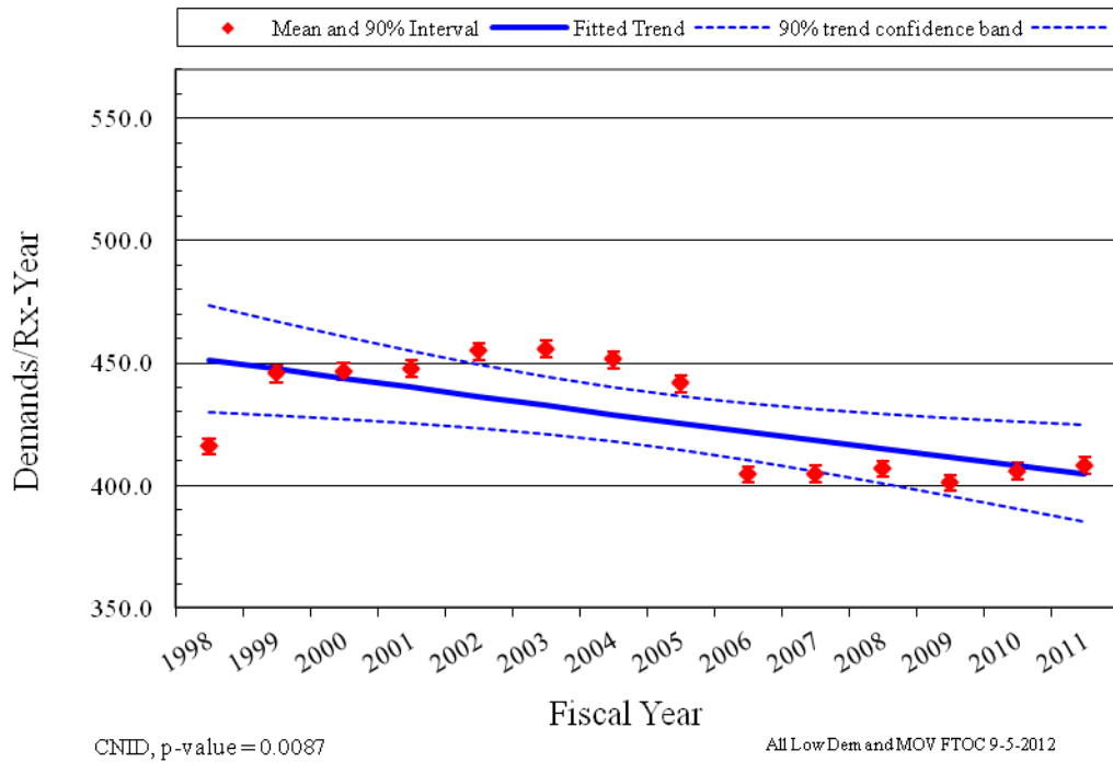
Figure 7. Frequency (demands per reactor year) of MOV operation demands, ≤ 20 demands per year.
