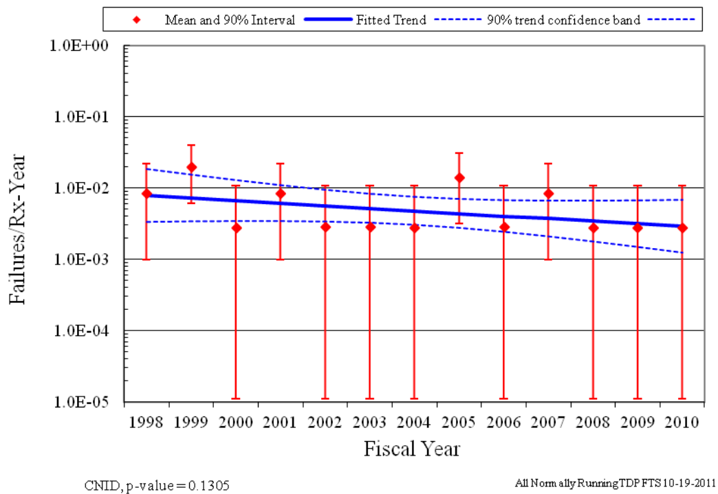
Figure 17. Frequency (events per reactor year) of FTS events, normally running TDPs.
