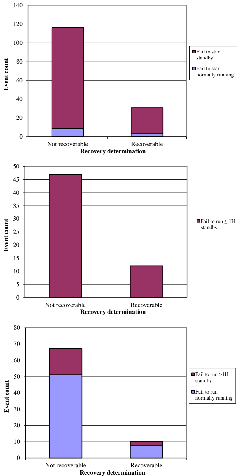
Figure 22. TDP failure event breakdown by recoverability determination, failure mode, and operational status.
