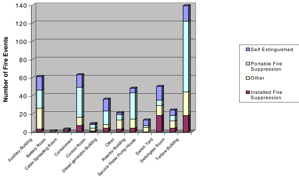
Figure 7. Distribution of fire events by plant location and method of suppression.
