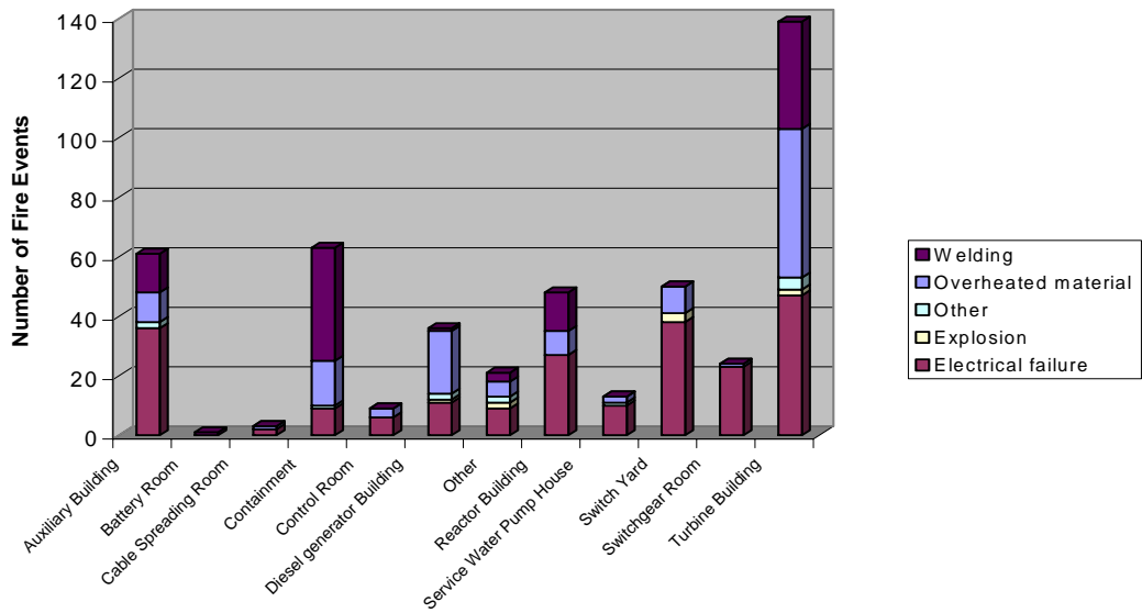
Figure 4. Distribution of fire events by plant location and fire discovery method.
