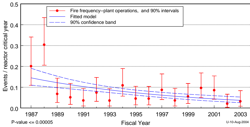
Figure 2. Fire events by fiscal year for plant at power.
