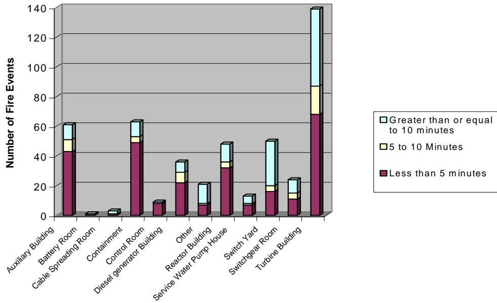
Figure 6. Distribution of fire events by plant location and fire duration.
