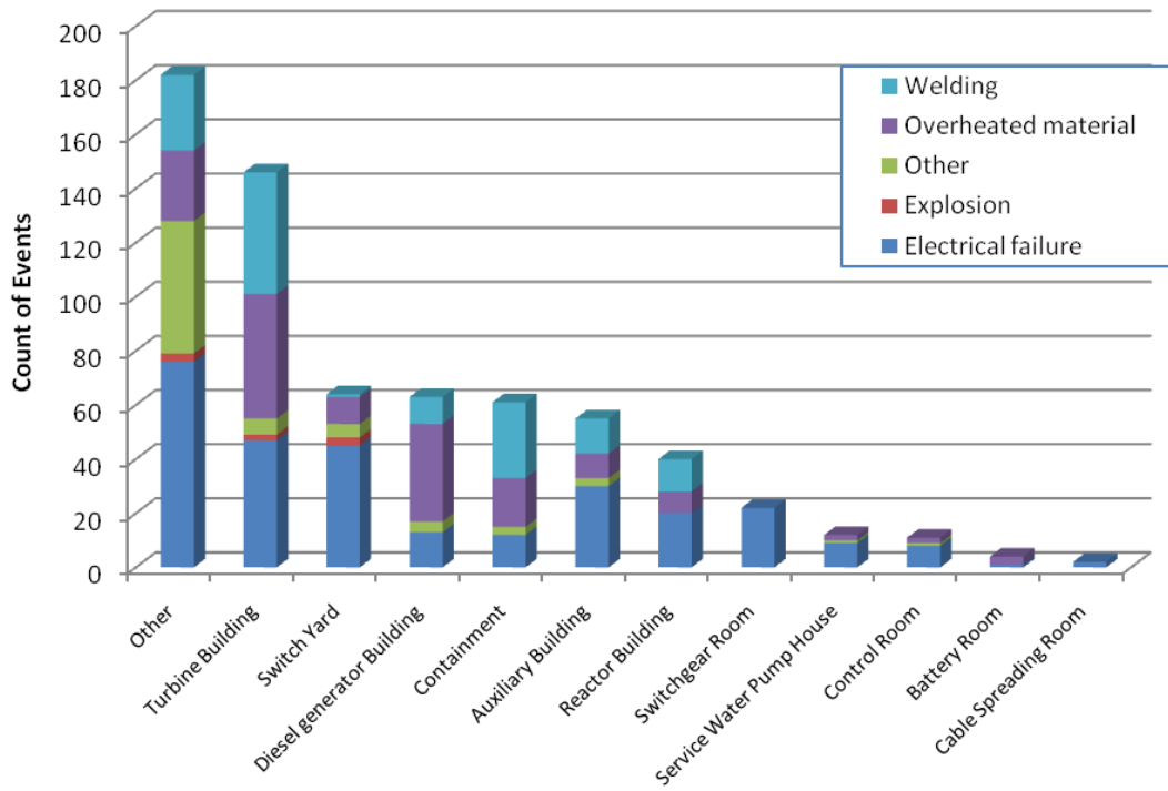
Figure 5. Distribution of fire events by plant location and cause.
