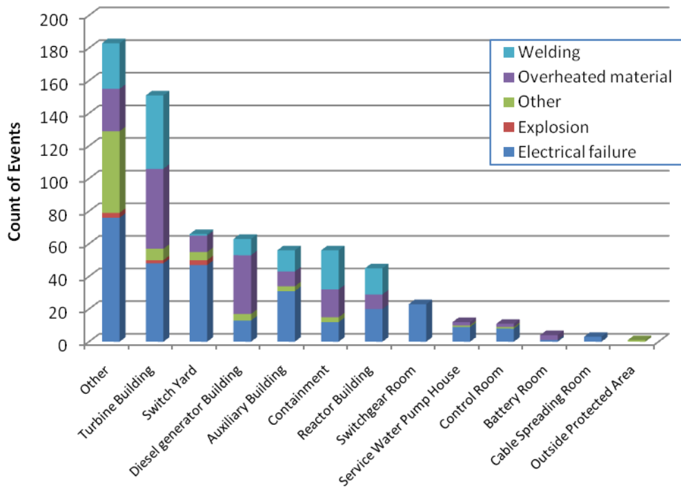
Figure 5. Distribution of fire events by plant location and cause.
