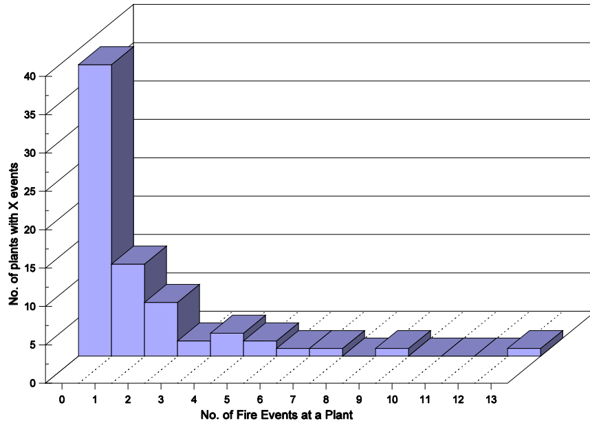
Figure A-2. Histogram of NEIL reported fires during shutdown
