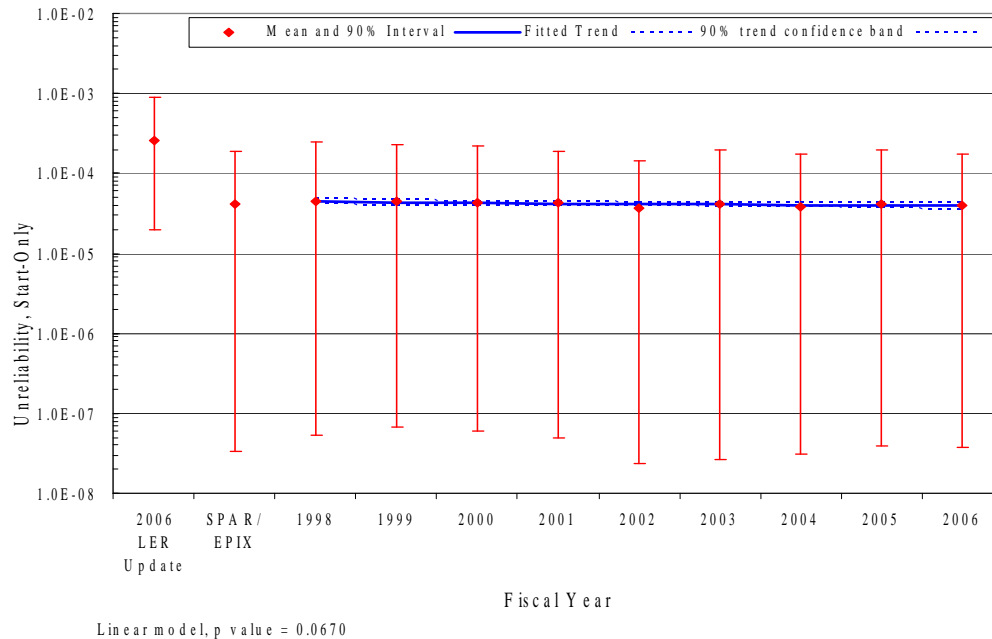
Figure 3. Trend of AFW system unreliability (start-only model), as a function of fiscal year.
