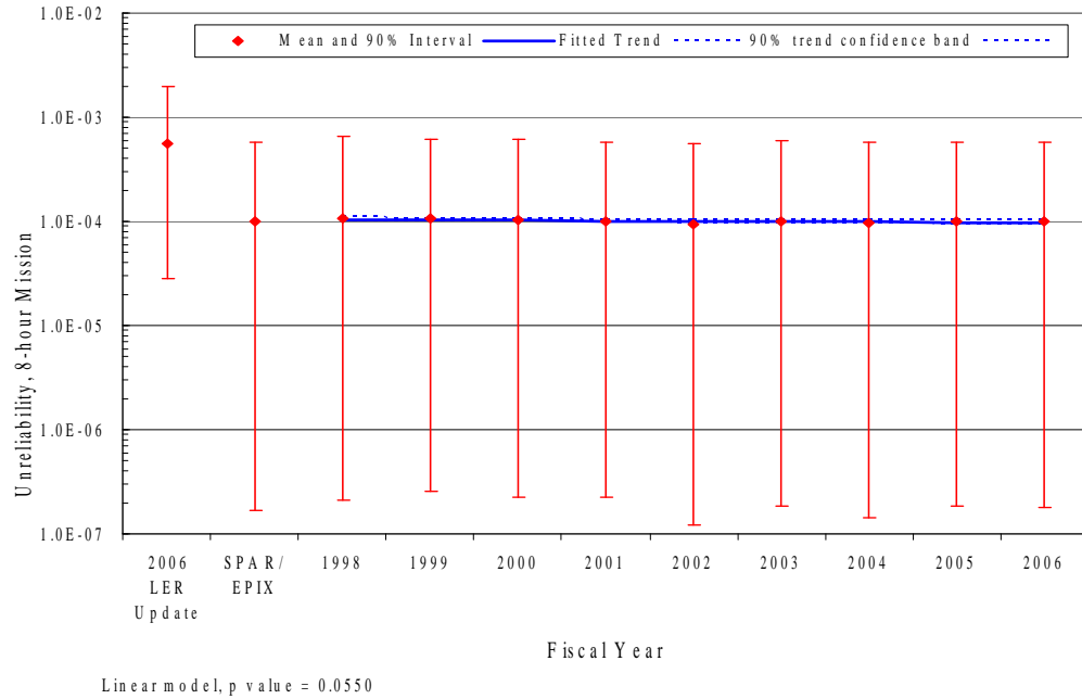
Figure 4. Trend of AFW system unreliability (8-hour model), as a function of fiscal year.
