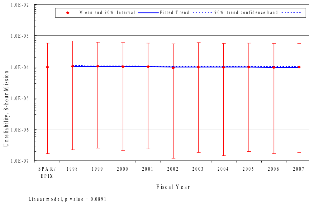
Figure 4. Trend of AFW system unreliability (8-hour model), as a function of fiscal year.
