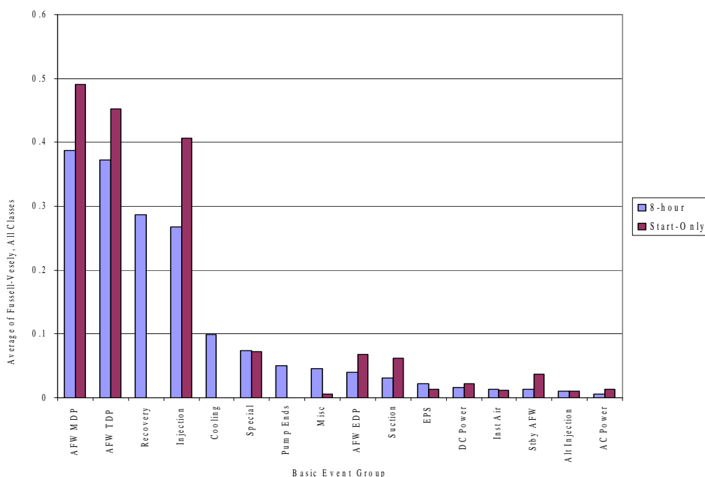
Figure 5. AFW industry-wide basic event group importances.
