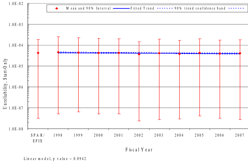
Figure 3. Trend of AFW system unreliability (start-only model), as a function of fiscal year.
