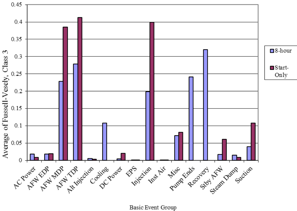
Figure 7. AFW Class 3 basic event group importances.
