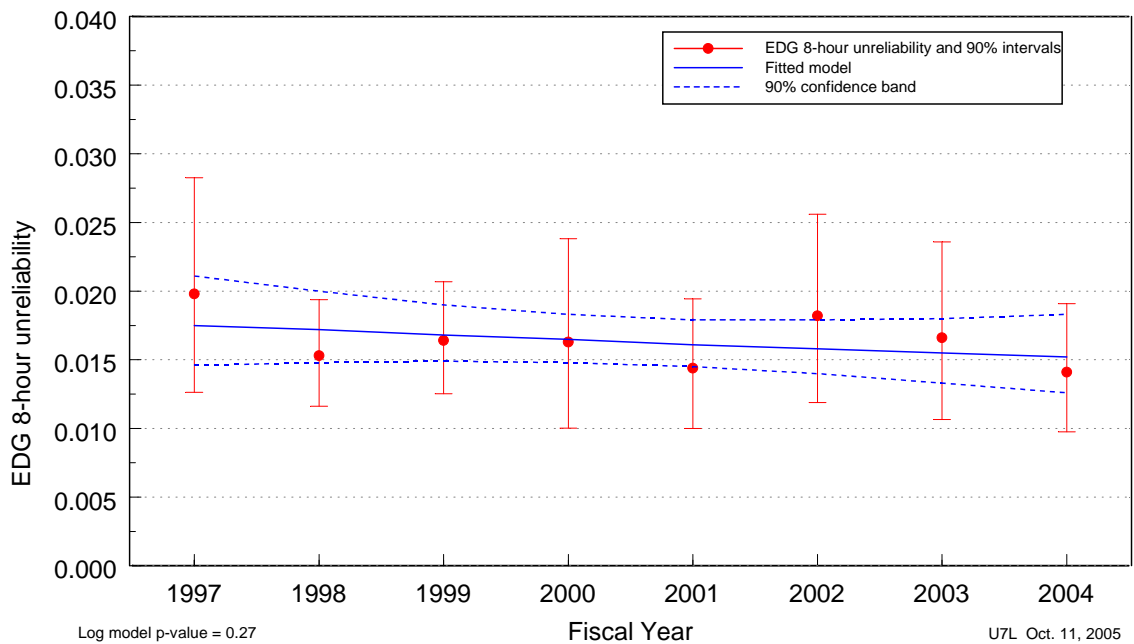
Figure 4. Trend of EDGs unreliability (8-hour model, with recovery), as a function of fiscal year.
