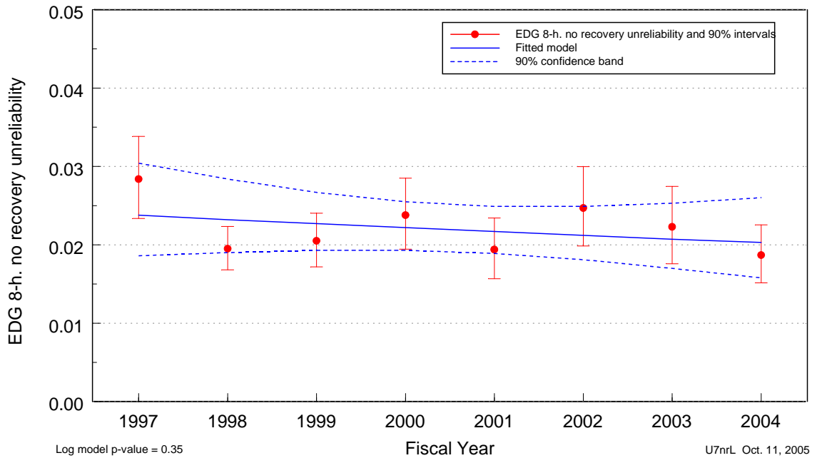
Figure 3. Trend of EDGs unreliability (8-hour model, no recovery), as a function of fiscal year.
