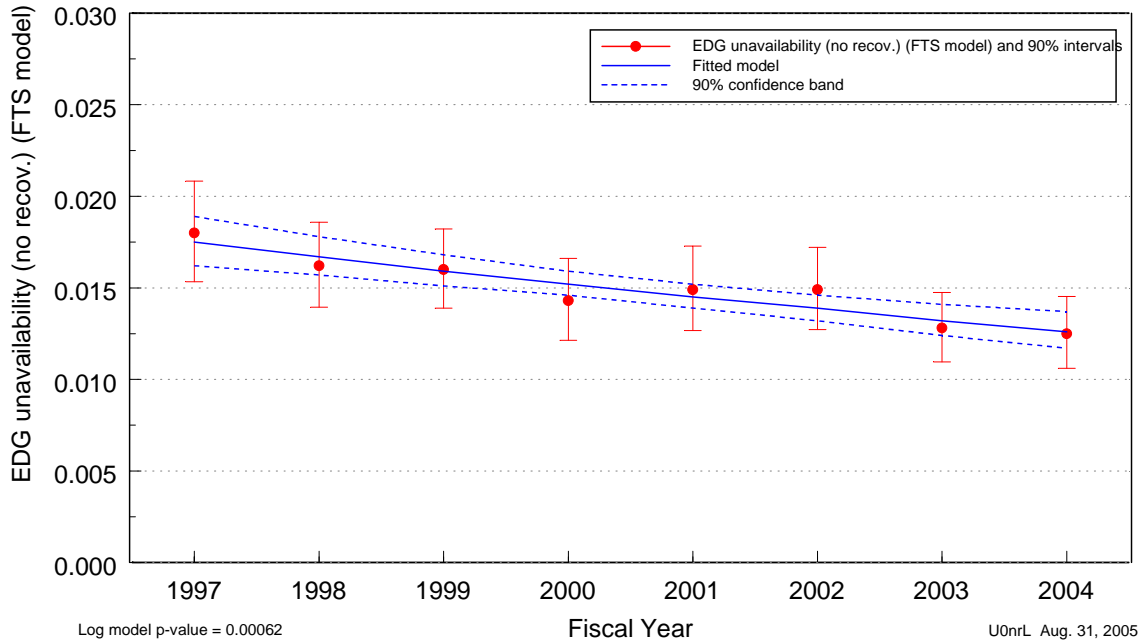
Figure 1. Trend of EDGs unavailability (FTS model, no recovery), as a function of fiscal year.
