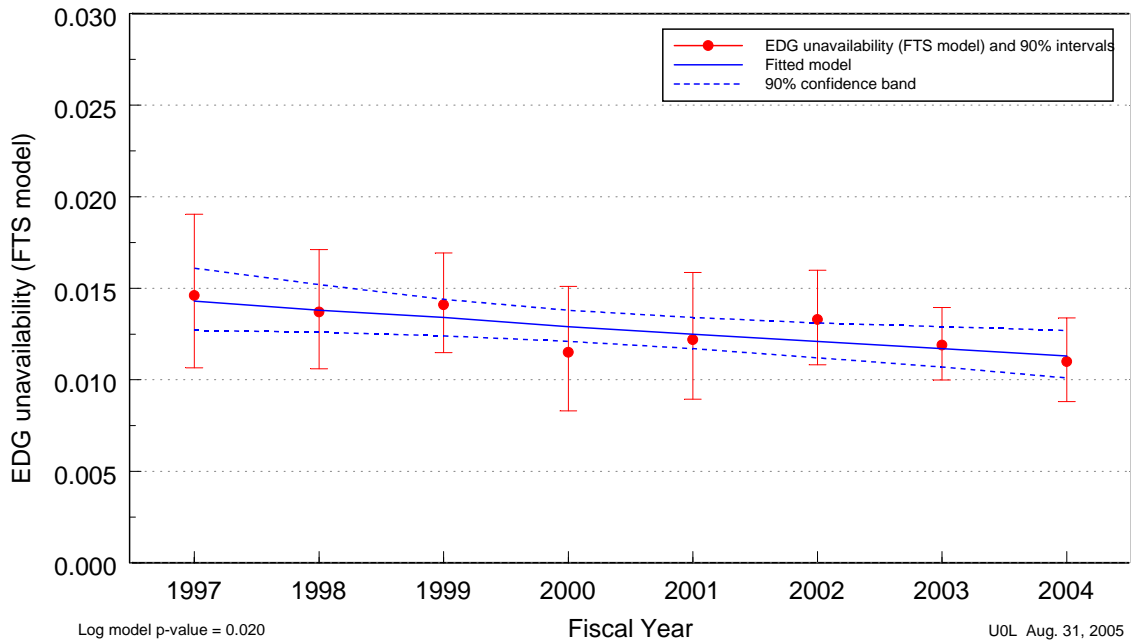
Figure 2. Trend of EDGs unavailability (FTS model, with recovery), as a function of fiscal year.
