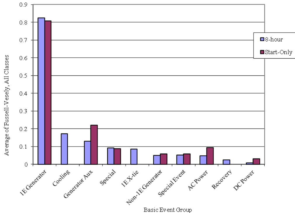
Figure 5. EPS industry-wide basic event group importances.
