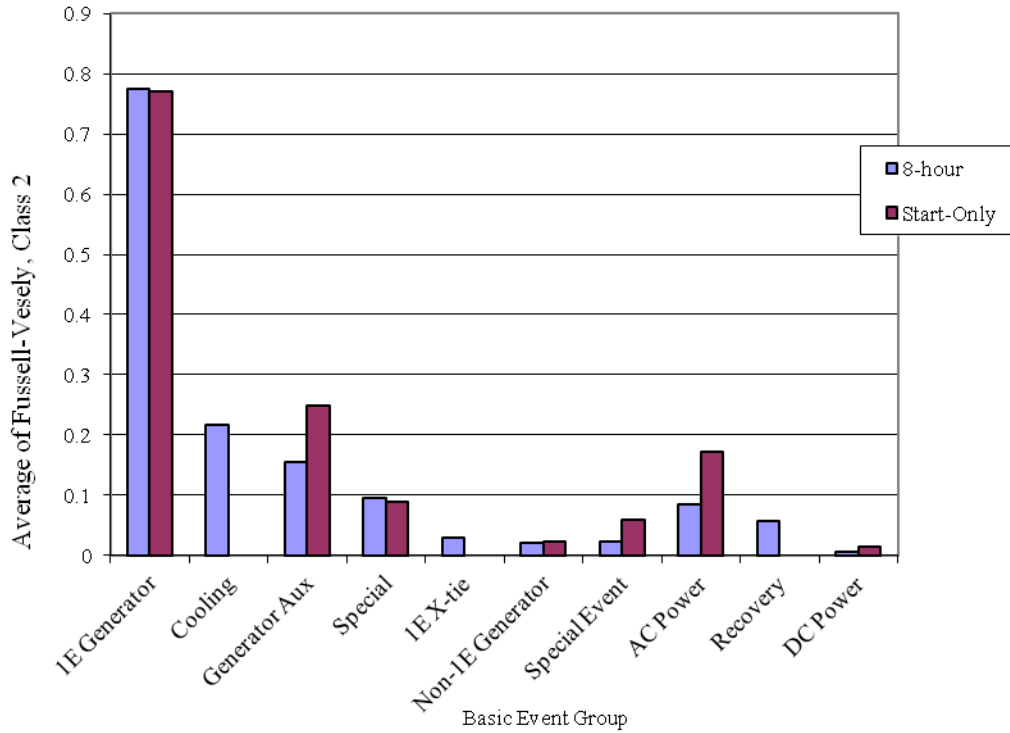
Figure 6. EPS Class 2 basic event group importances.
