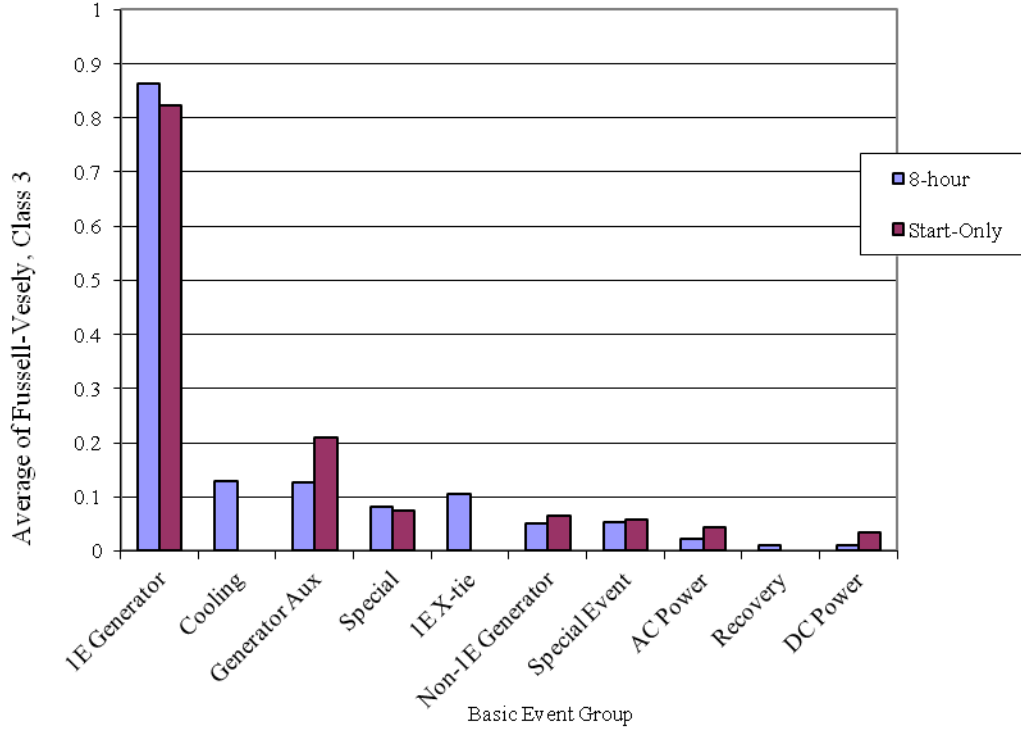
Figure 7. EPS Class 3 basic event group importances.
