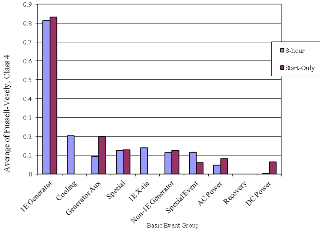
Figure 8. EPS Class 4 basic event group importances.
