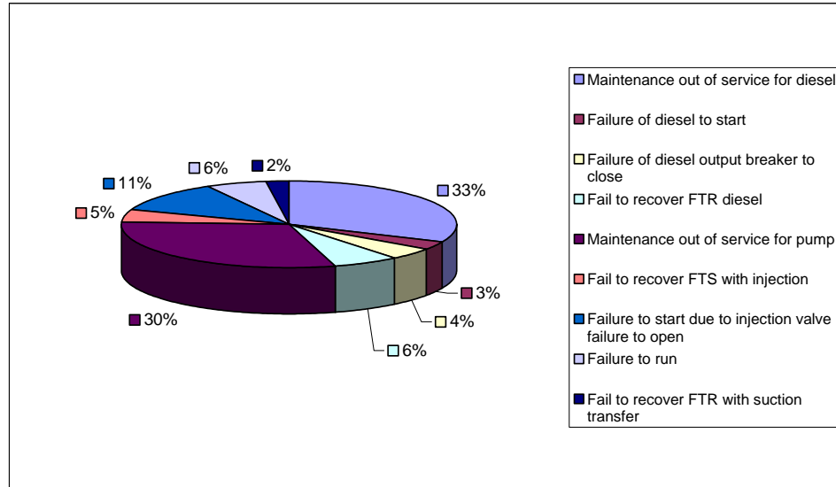
Figure 6. Segment failure distribution, 8-hour mission.
