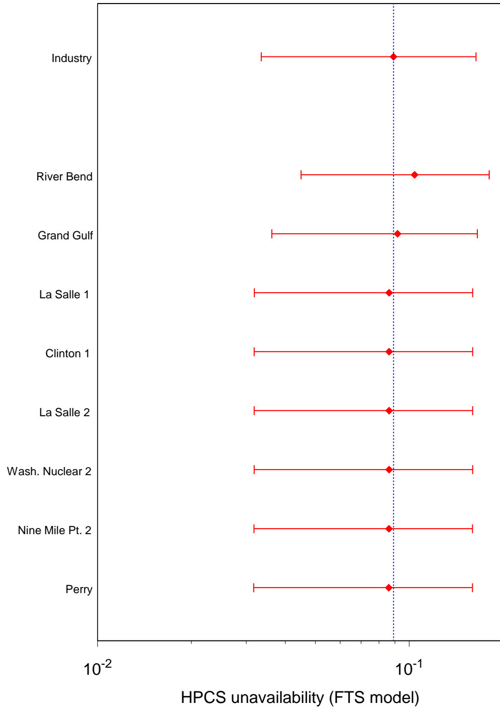
Figure 1. Plant-specific estimates of HPCS system unavailability for FTS model.
