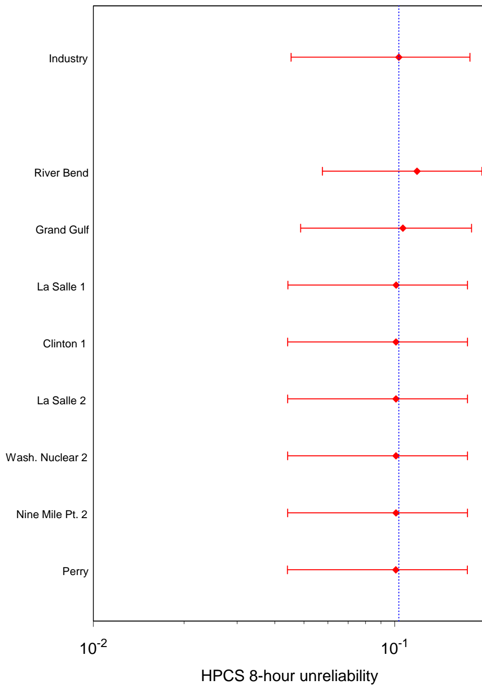
Figure 4. Plant-specific estimates of HPCS system unreliability for an 8-hour mission.
