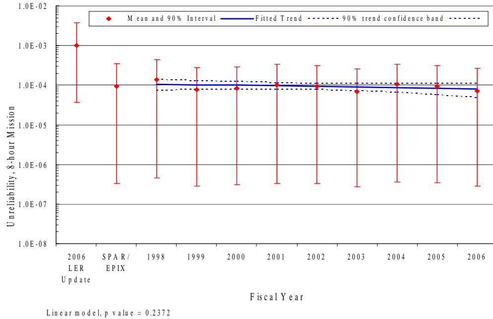
Figure 4. Trend of HPSI system unreliability (8-hour model), as a function of fiscal year.
