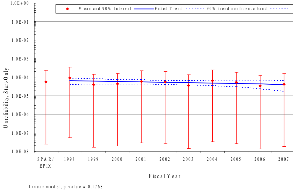
Figure 3. Trend of HPSI system unreliability (start-only model), as a function of fiscal year.
