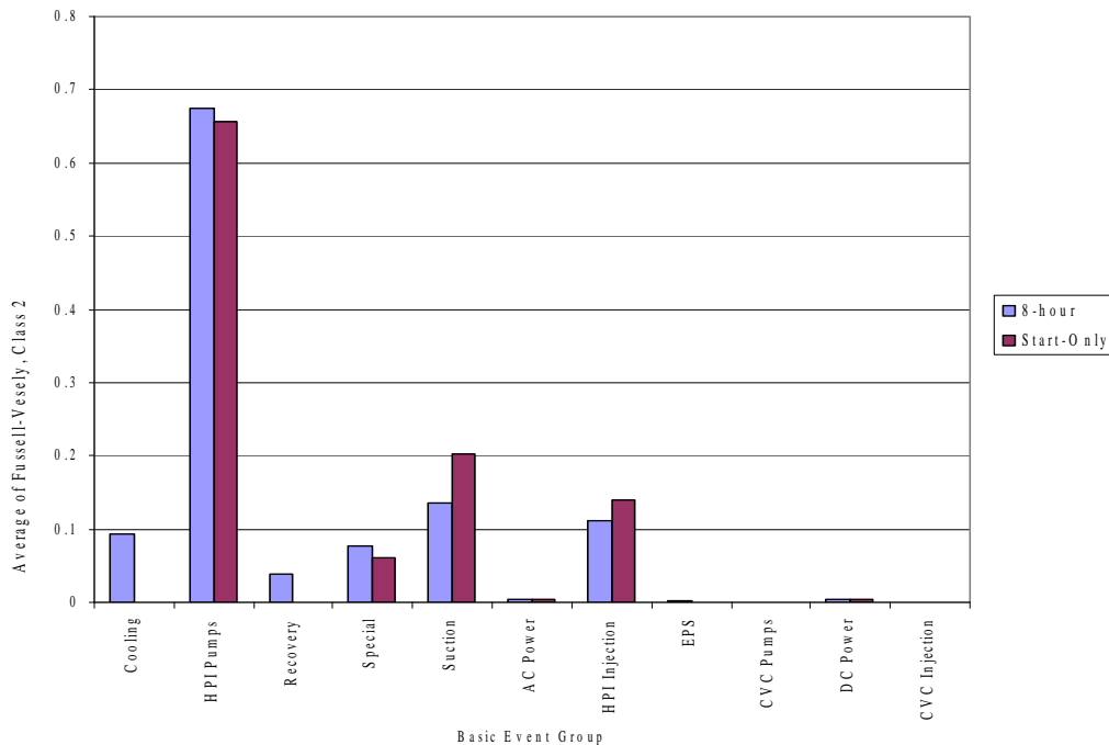
Figure 6. HPSI Class 2 basic event group importances.
