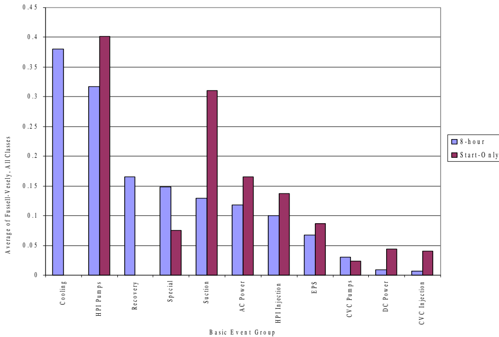
Figure 5. HPSI industry-wide basic event group importances.
