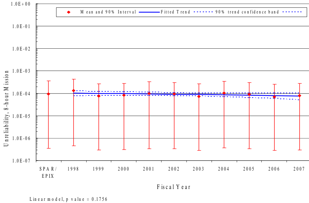
Figure 4. Trend of HPSI system unreliability (8-hour model), as a function of fiscal year.
