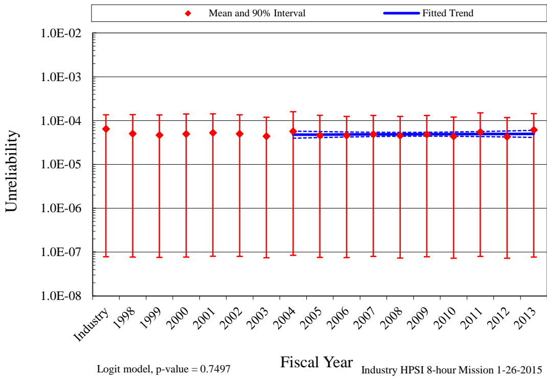
Figure 4. Trend of HPSI system unreliability (8-hour model), as a function of fiscal year.
