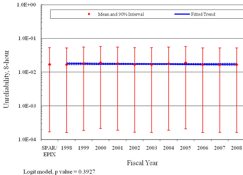
Figure 1. Trend of ISO system unreliability (operate and makeup), as a function of fiscal year.
