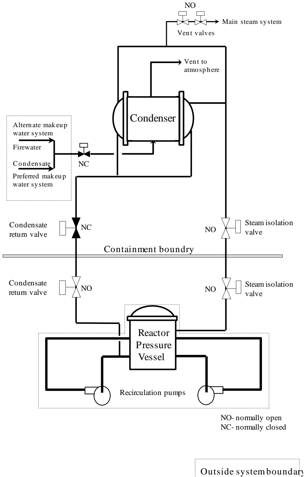
Figure 3. Simplified single train isolation condenser system schematic.
